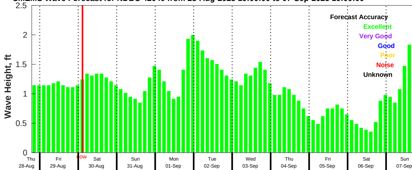
CMEMS Wave Forecast for NDBC 42040 from 28-Aug-2025 19:00:00 to 07-Sep-2025 19:00:00
