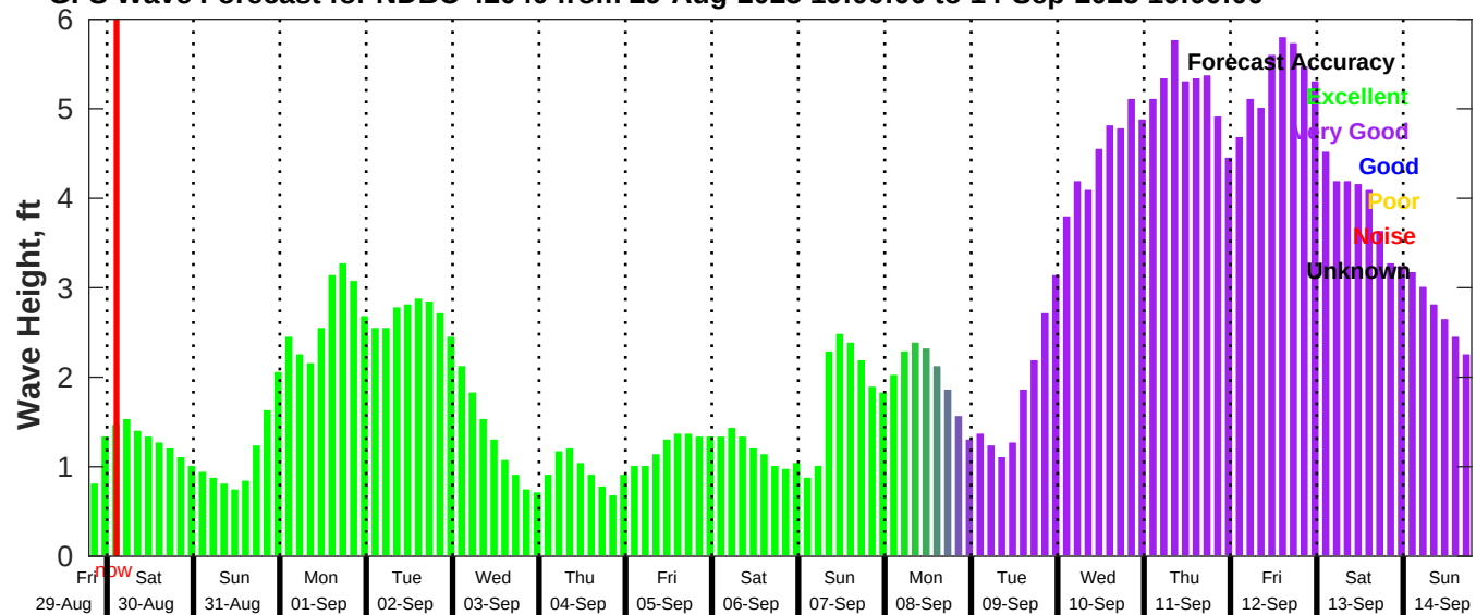
GFS Wave Forecast for NDBC 42040 from 29-Aug-2025 19:00:00 to 14-Sep-2025 19:00:00
