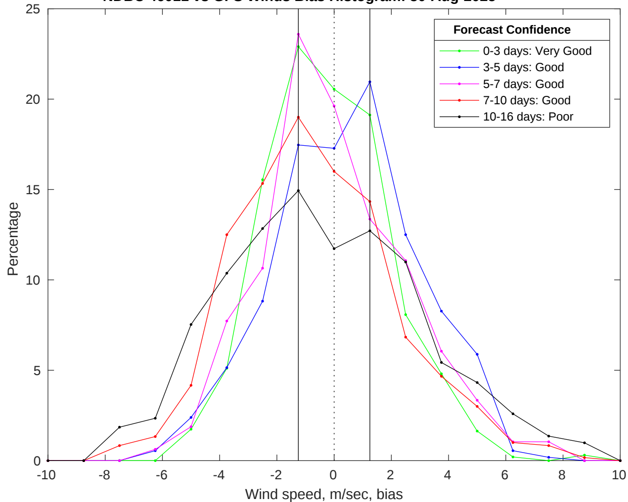
NDBC 46011 vs GFS Winds Bias Histogram: 30-Aug-2025
