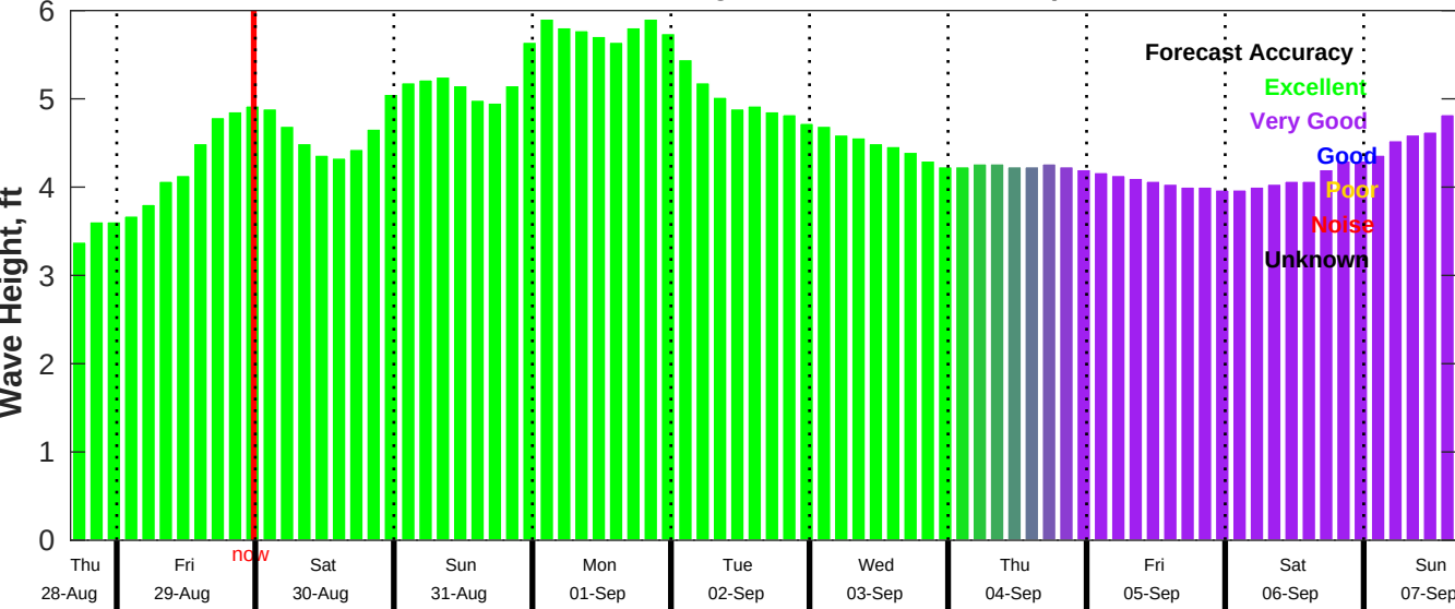
CMEMS Wave Forecast for NDBC 46011 from 28-Aug-2025 16:00:00 to 07-Sep-2025 16:00:00
