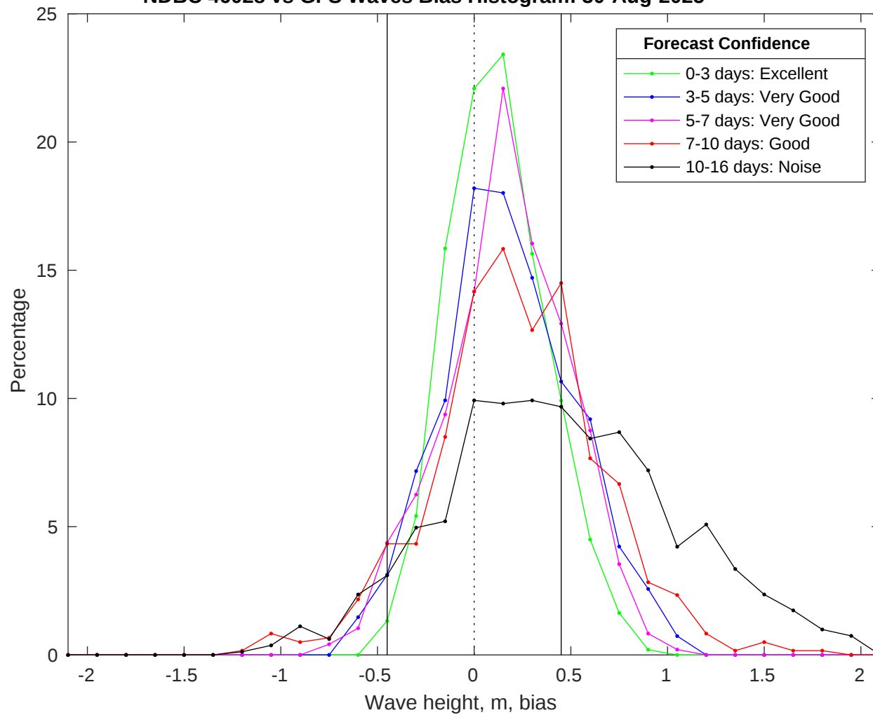
NDBC 46028 vs GFS Waves Bias Histogram: 30-Aug-2025
