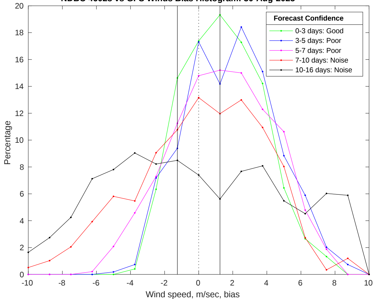
NDBC 46028 vs GFS Winds Bias Histogram: 30-Aug-2025
