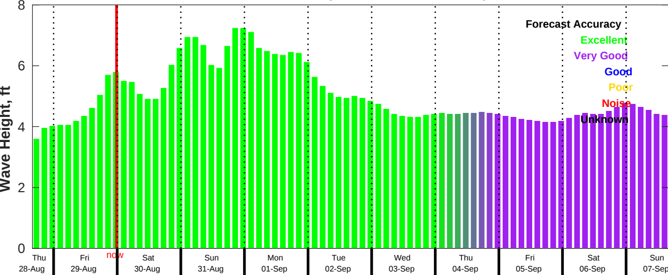
CMEMS Wave Forecast for NDBC 46028 from 28-Aug-2025 16:00:00 to 07-Sep-2025 16:00:00
