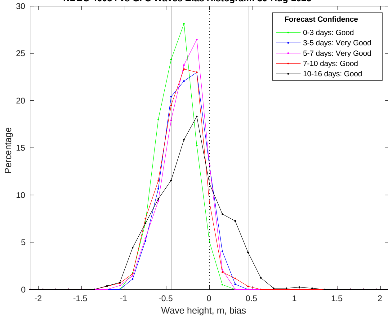
NDBC 46054 vs GFS Waves Bias Histogram: 30-Aug-2025
