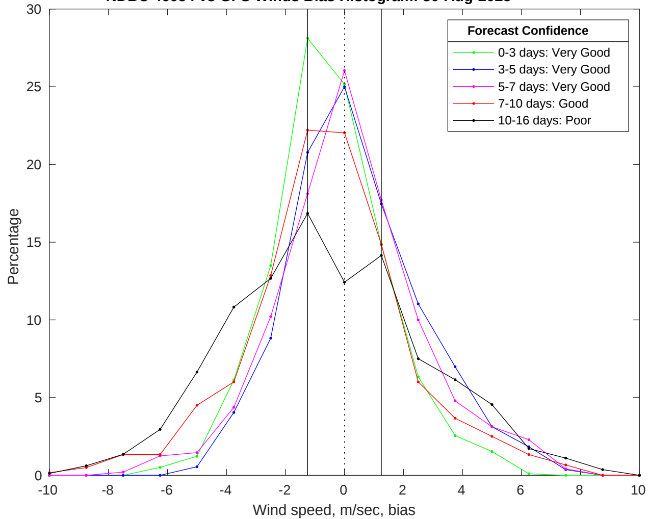
NDBC 46054 vs GFS Winds Bias Histogram: 30-Aug-2025
