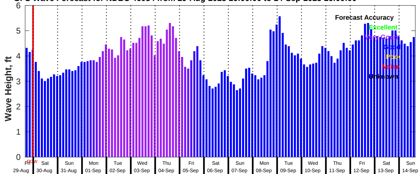
GFS Wave Forecast for NDBC 46054 from 29-Aug-2025 16:00:00 to 14-Sep-2025 16:00:00
