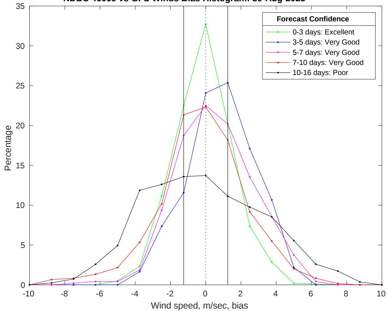
NDBC 46069 vs GFS Winds Bias Histogram: 30-Aug-2025
