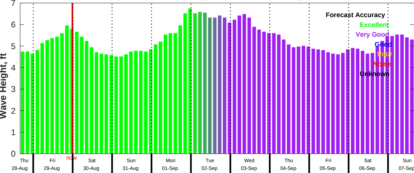
CMEMS Wave Forecast for NDBC 46069 from 28-Aug-2025 16:00:00 to 07-Sep-2025 16:00:00
