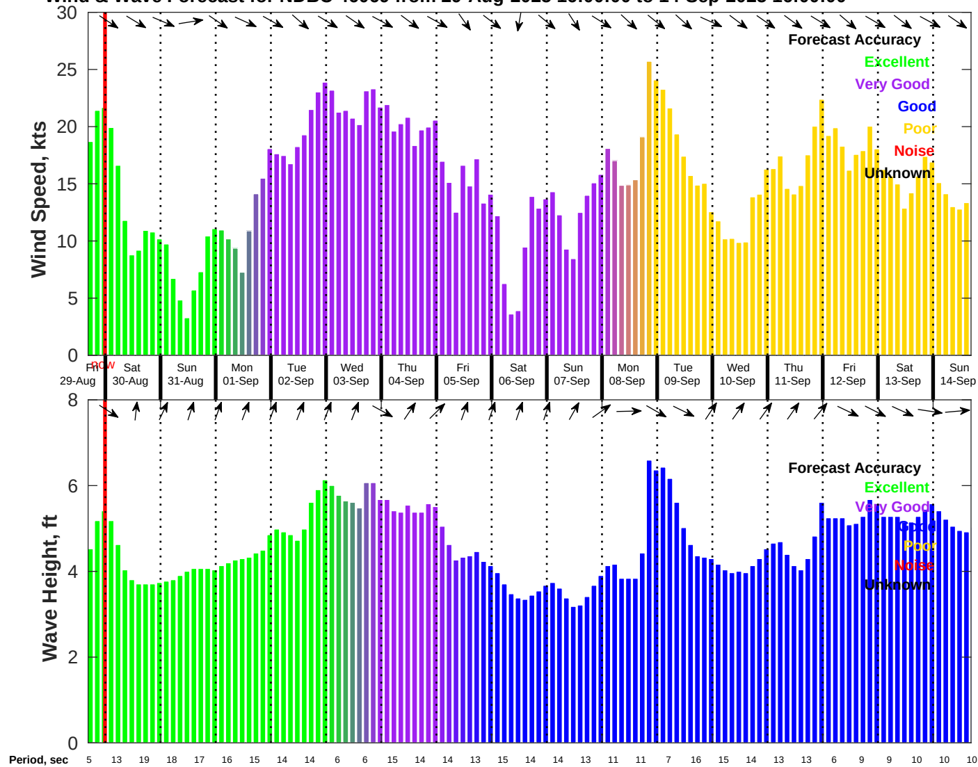
Wind & Wave Forecast for NDBC 46069 from 29-Aug-2025 16:00:00 to 14-Sep-2025 16:00:00
