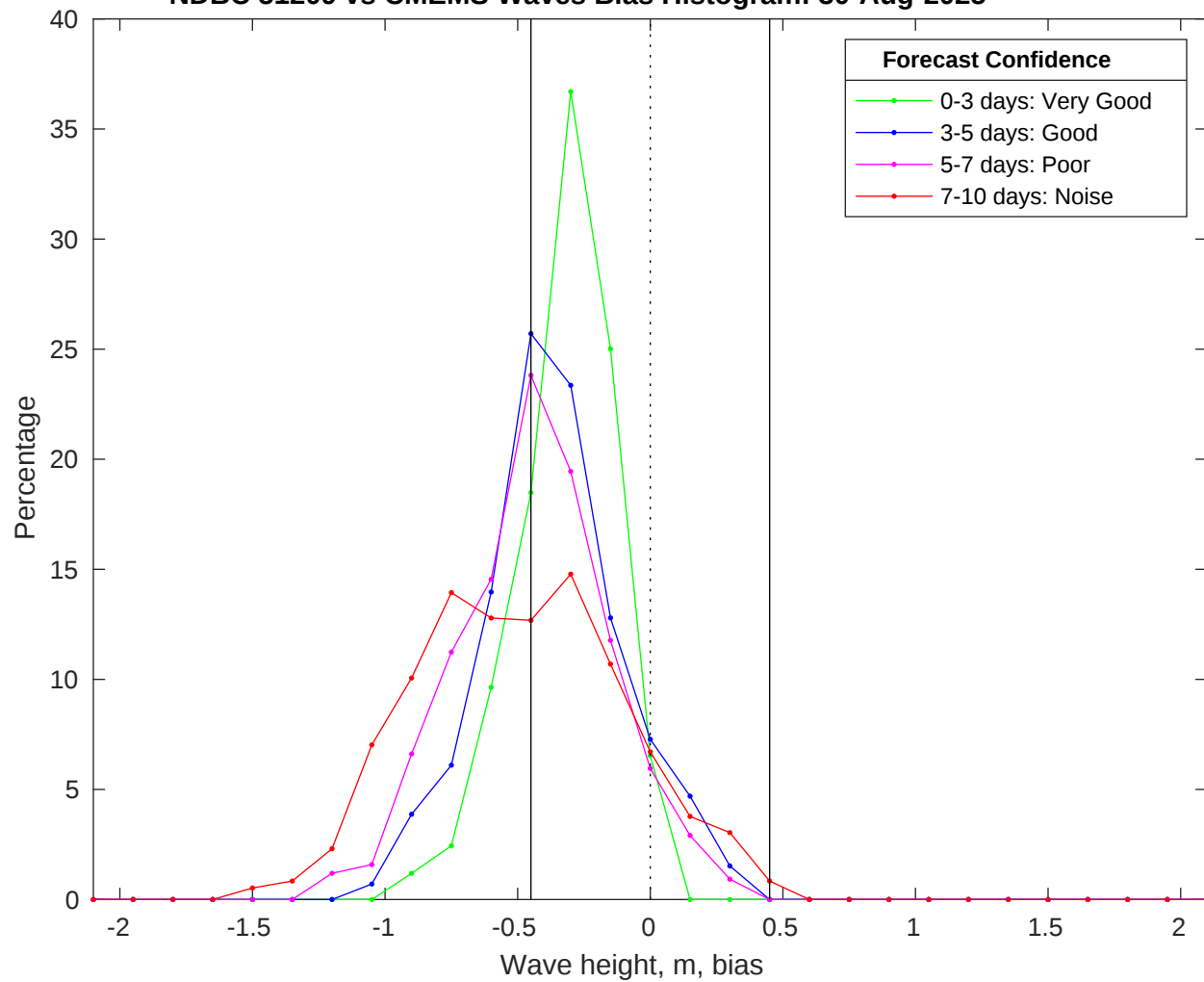
NDBC 51209 vs CMEMS Waves Bias Histogram: 30-Aug-2025
