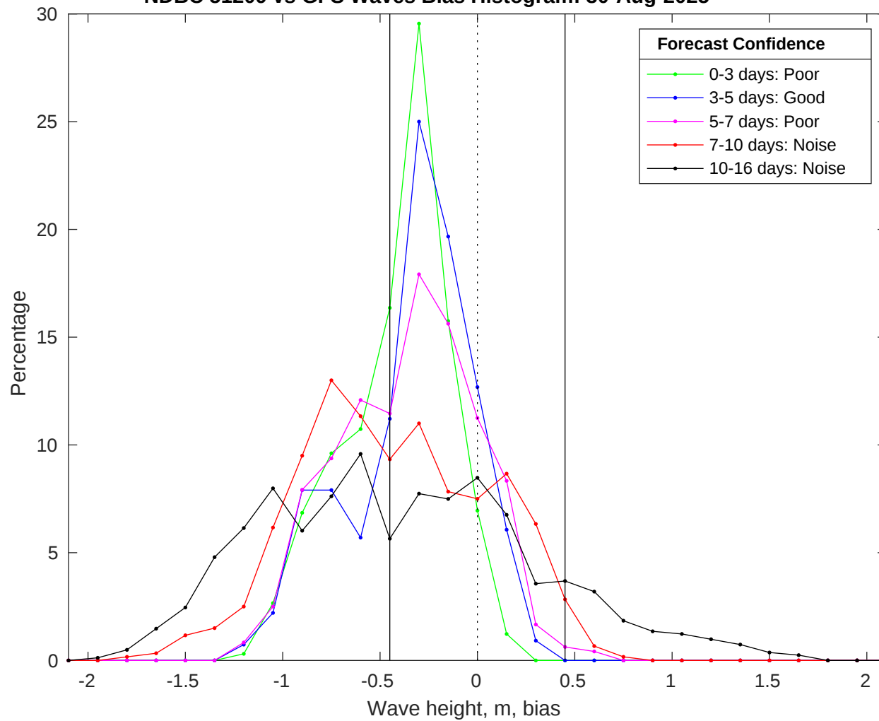
NDBC 51209 vs GFS Waves Bias Histogram: 30-Aug-2025
