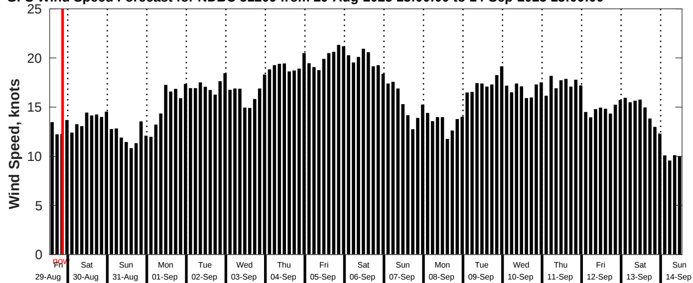
GFS Wind Speed Forecast for NDBC 51209 from 29-Aug-2025 13:00:00 to 14-Sep-2025 13:00:00
