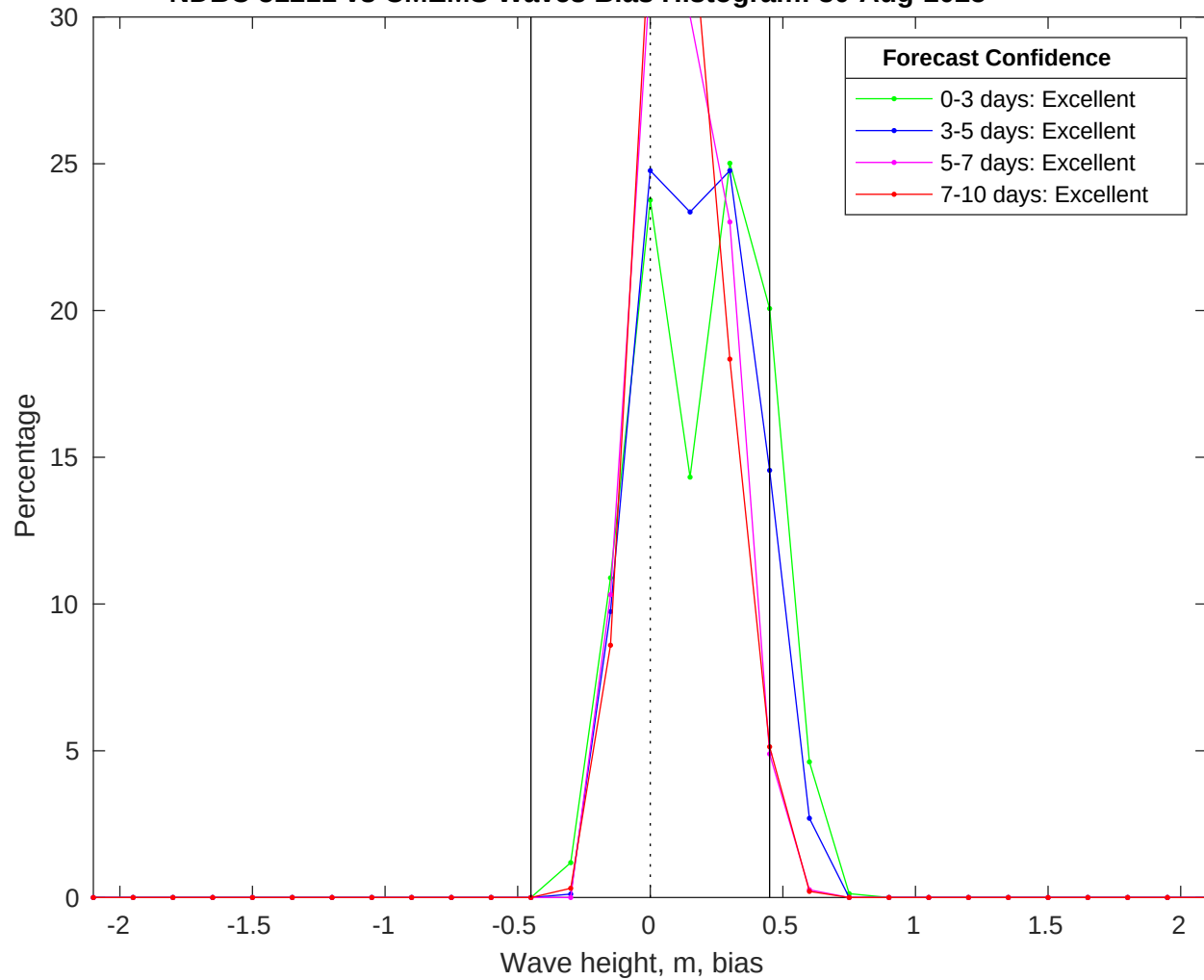
NDBC 51211 vs CMEMS Waves Bias Histogram: 30-Aug-2025
