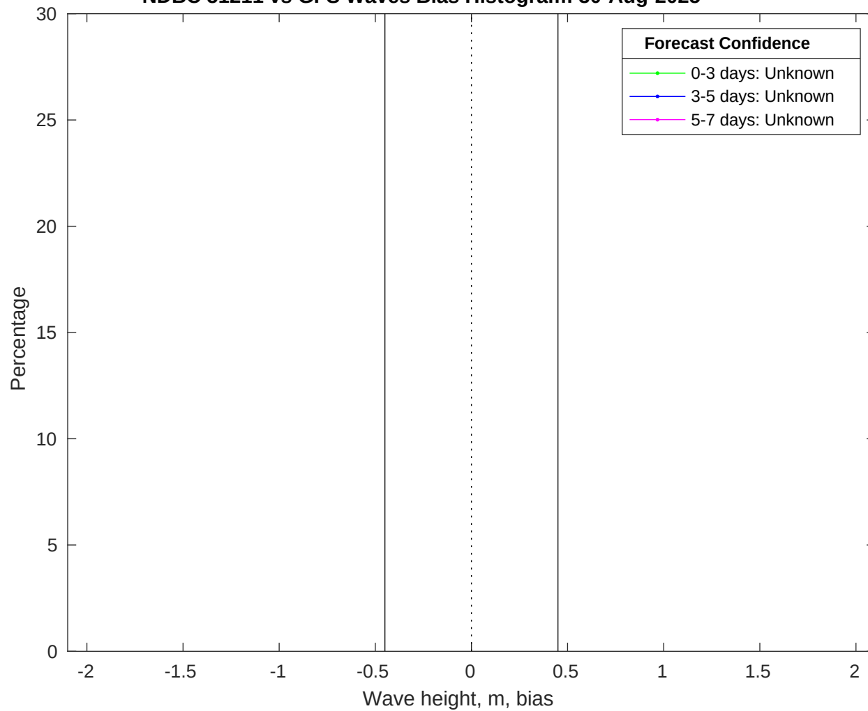
NDBC 51211 vs GFS Waves Bias Histogram: 30-Aug-2025
