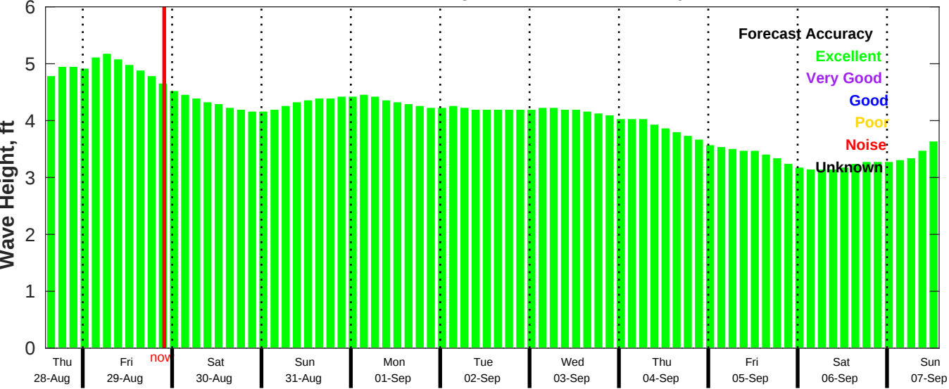
CMEMS Wave Forecast for NDBC 51211 from 28-Aug-2025 14:00:00 to 07-Sep-2025 14:00:00
