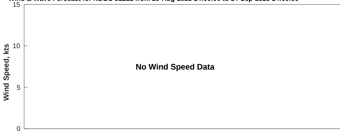
Wind & Wave Forecast for NDBC 51211 from 29-Aug-2025 14:00:00 to 14-Sep-2025 14:00:00
