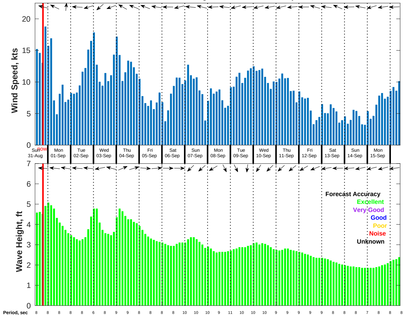
Wind & Wave Forecast for NDBC 52211 from 30-Aug-2025 11:00:00 to 15-Sep-2025 11:00:00
