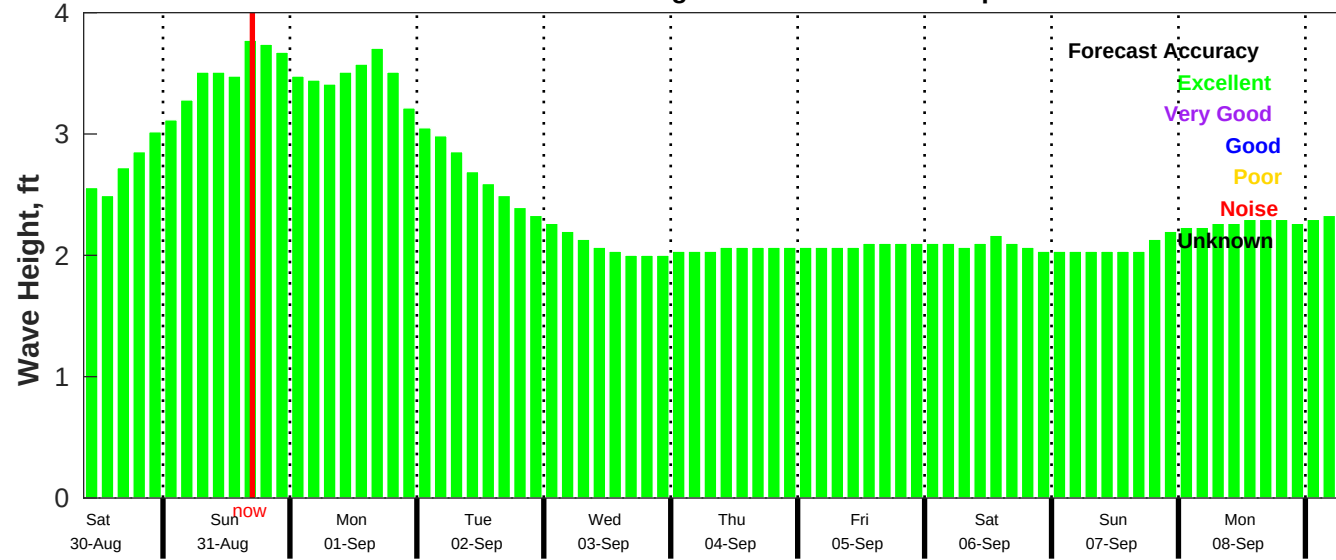
CMEMS Wave Forecast for NDBC 52212 from 29-Aug-2025 09:00:00 to 08-Sep-2025 09:00:00
