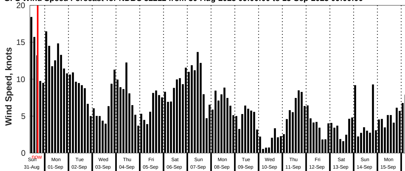
GFS Wind Speed Forecast for NDBC 52212 from 30-Aug-2025 09:00:00 to 15-Sep-2025 09:00:00
