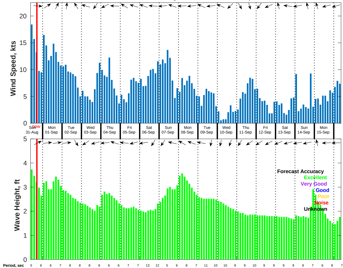
Wind & Wave Forecast for NDBC 52212 from 30-Aug-2025 09:00:00 to 15-Sep-2025 09:00:00
