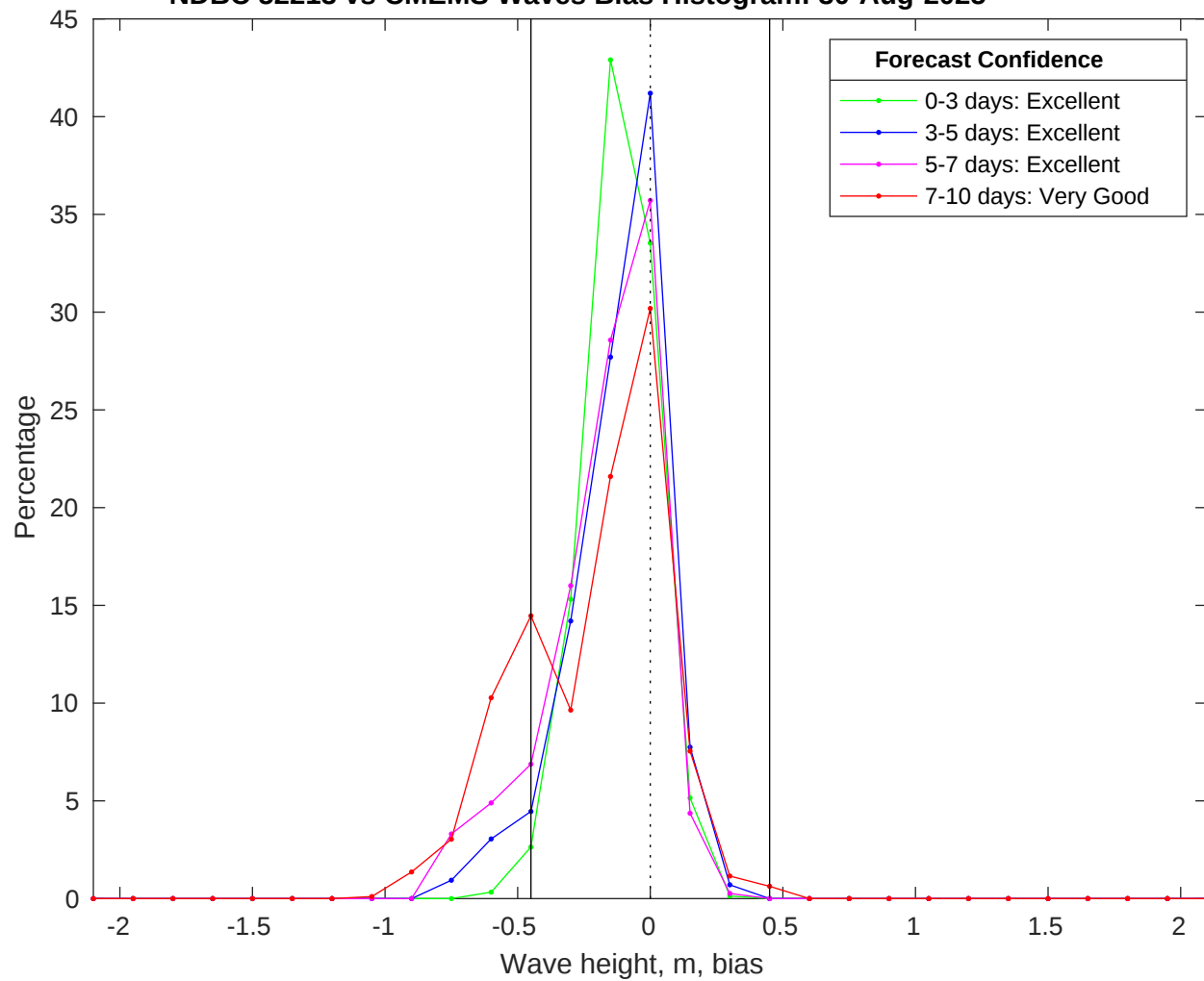
NDBC 52213 vs CMEMS Waves Bias Histogram: 30-Aug-2025
