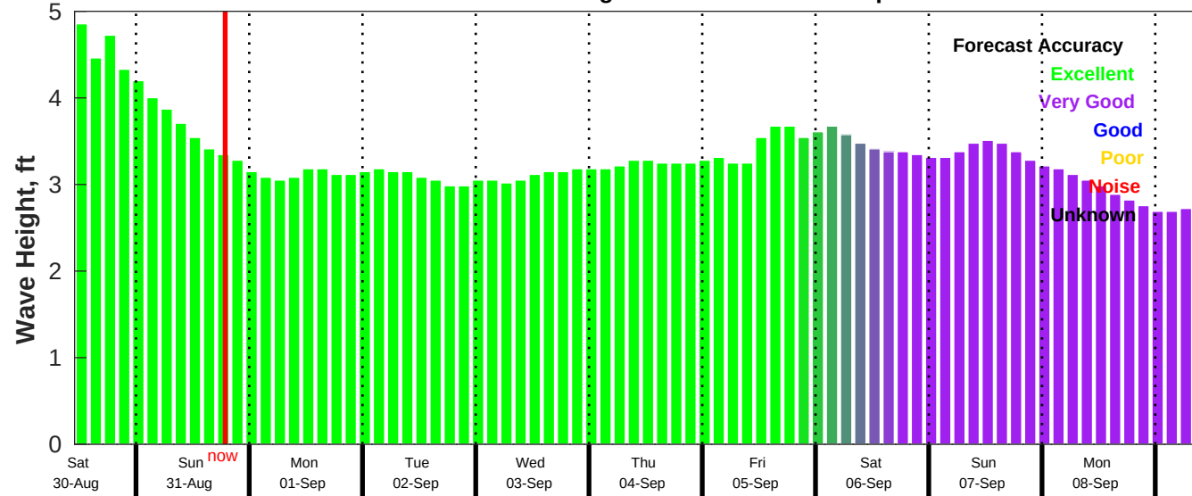
CMEMS Wave Forecast for NDBC 52213 from 29-Aug-2025 11:00:00 to 08-Sep-2025 11:00:00
