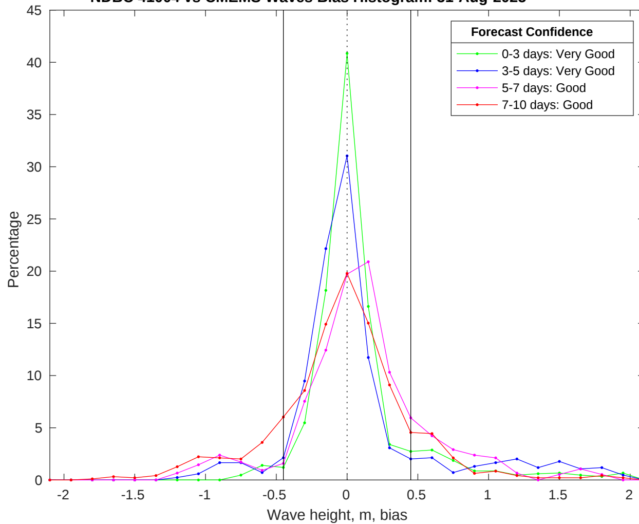
NDBC 41004 vs CMEMS Waves Bias Histogram: 31-Aug-2025
