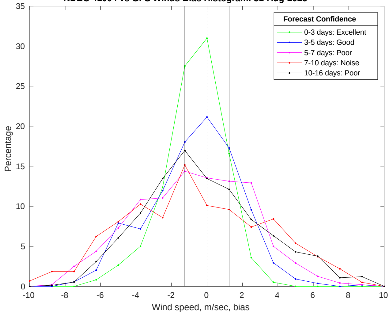
NDBC 41004 vs GFS Winds Bias Histogram: 31-Aug-2025
