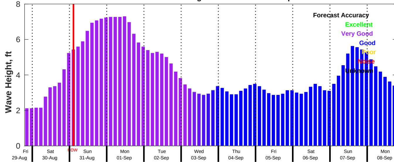
CMEMS Wave Forecast for NDBC 41004 from 29-Aug-2025 19:00:00 to 08-Sep-2025 19:00:00
