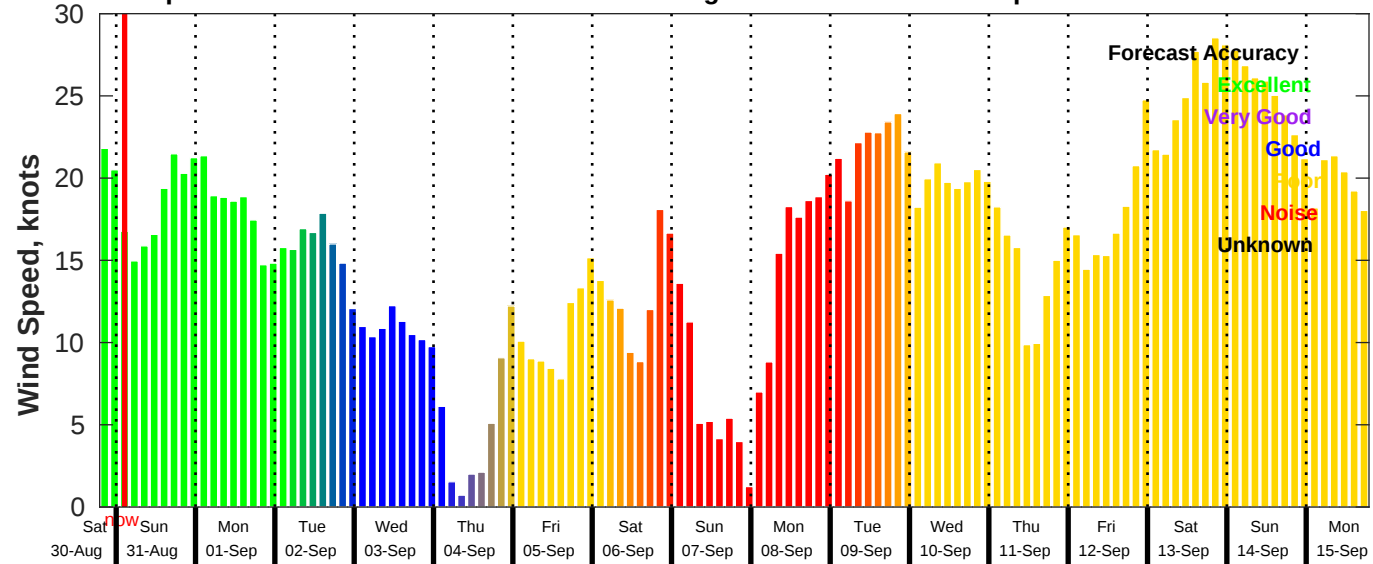
GFS Wind Speed Forecast for NDBC 41004 from 30-Aug-2025 19:00:00 to 15-Sep-2025 19:00:00
