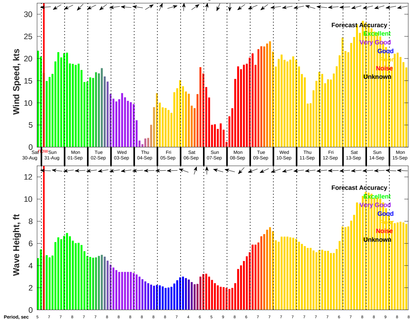
Wind & Wave Forecast for NDBC 41004 from 30-Aug-2025 19:00:00 to 15-Sep-2025 19:00:00
