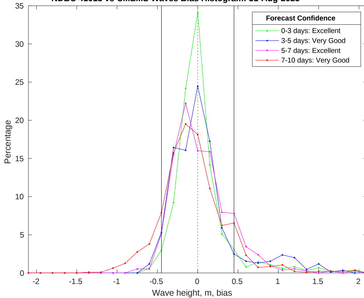
NDBC 41013 vs CMEMS Waves Bias Histogram: 31-Aug-2025
