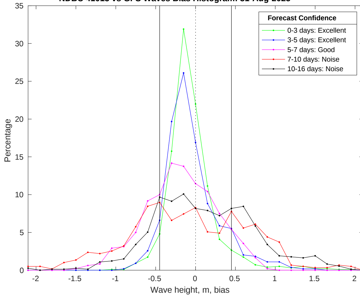
NDBC 41013 vs GFS Waves Bias Histogram: 31-Aug-2025
