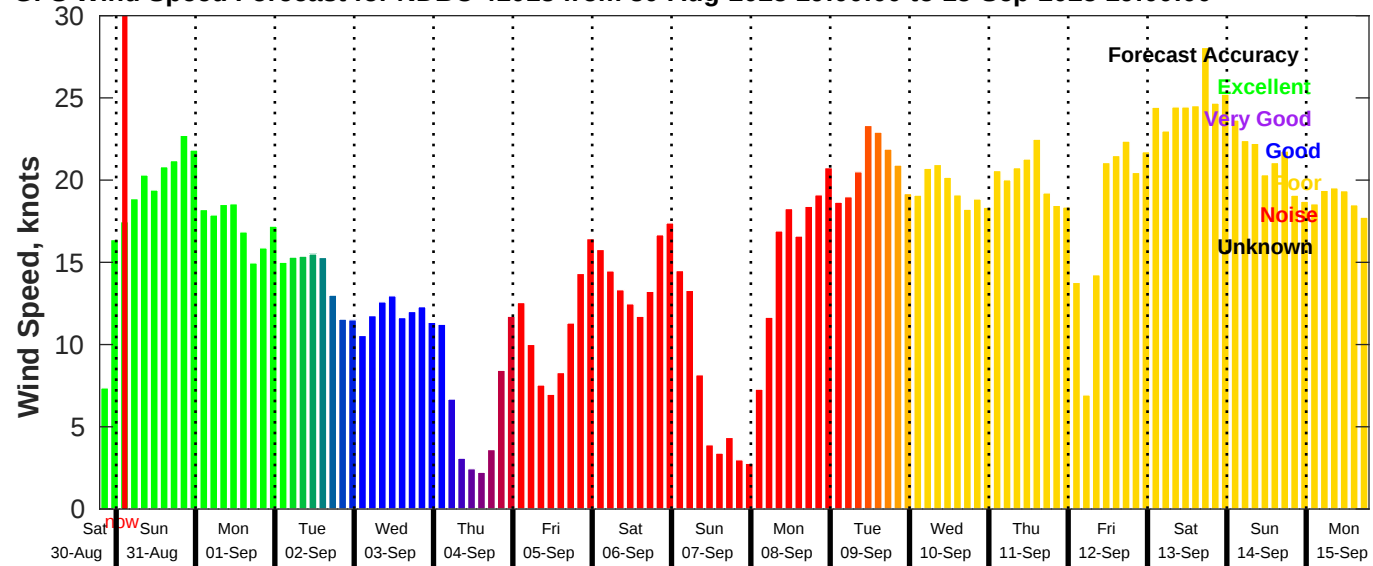
GFS Wind Speed Forecast for NDBC 41013 from 30-Aug-2025 19:00:00 to 15-Sep-2025 19:00:00
