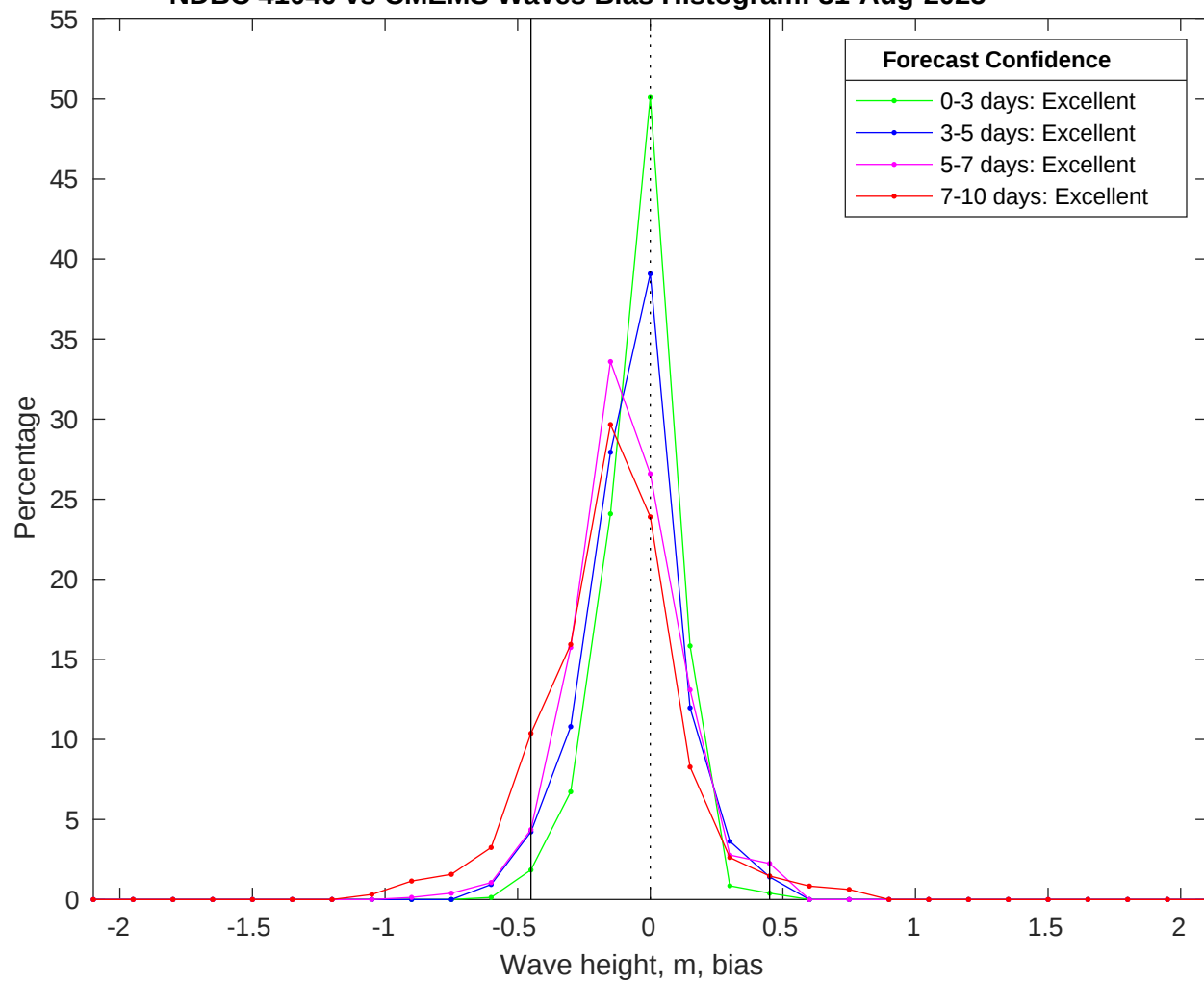
NDBC 41040 vs CMEMS Waves Bias Histogram: 31-Aug-2025
