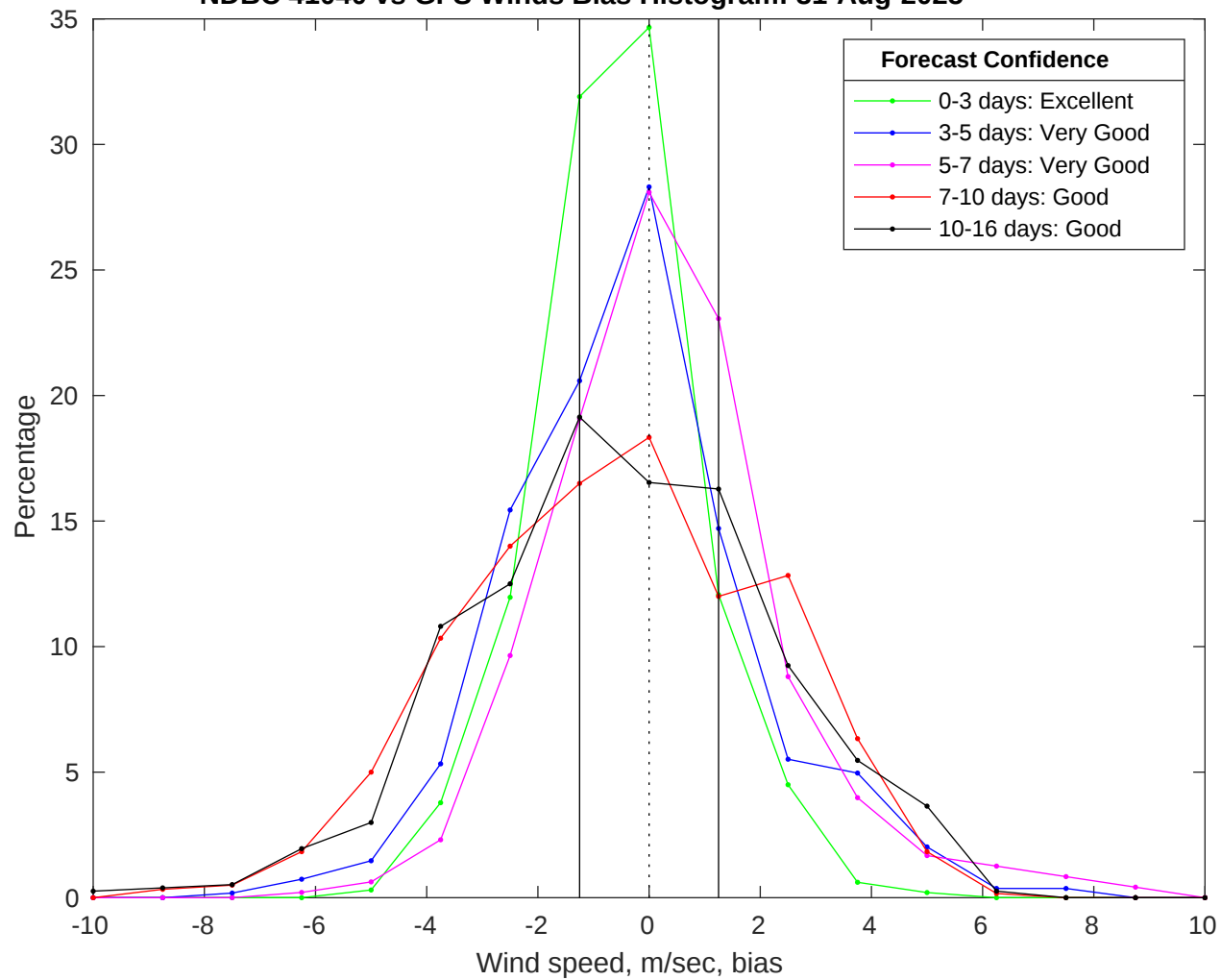
NDBC 41040 vs GFS Winds Bias Histogram: 31-Aug-2025
