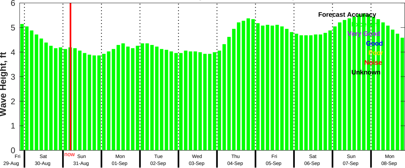
CMEMS Wave Forecast for NDBC 41040 from 29-Aug-2025 21:00:00 to 08-Sep-2025 21:00:00
