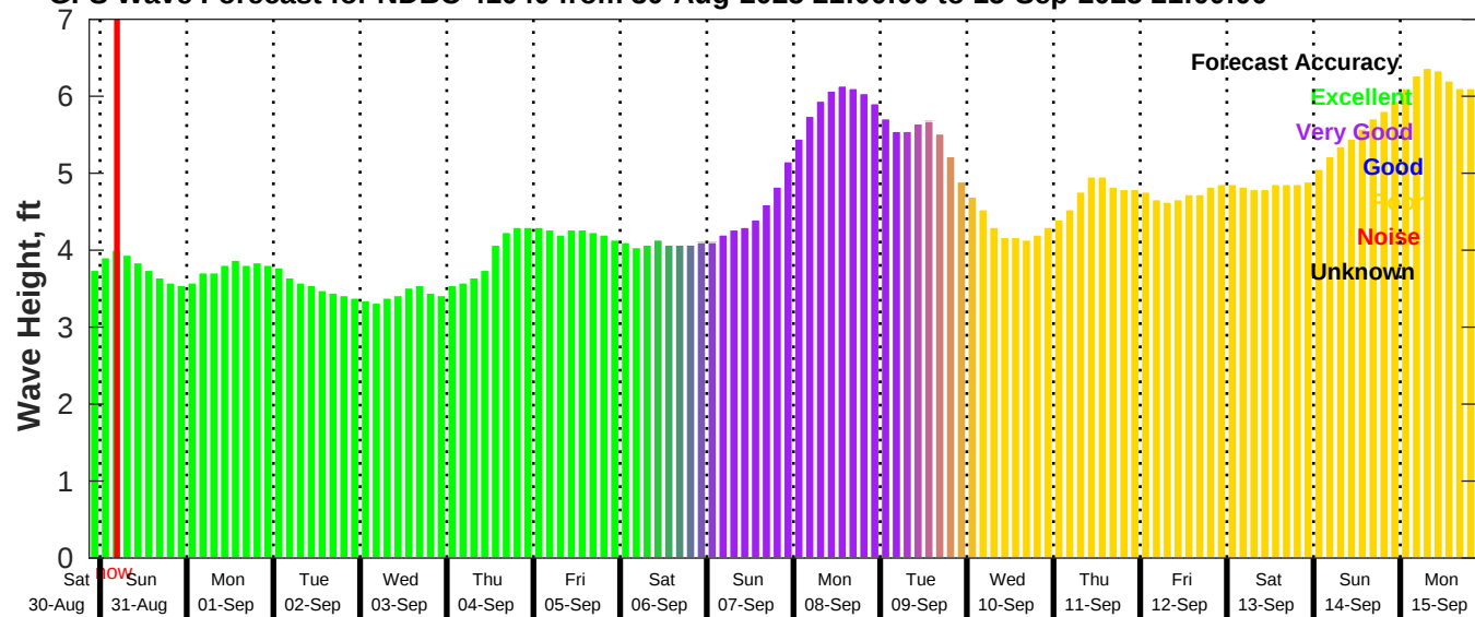
GFS Wave Forecast for NDBC 41040 from 30-Aug-2025 21:00:00 to 15-Sep-2025 21:00:00
