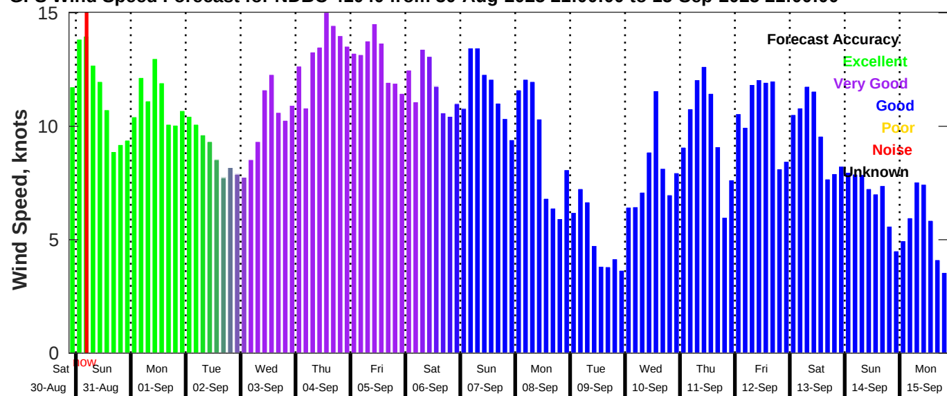
GFS Wind Speed Forecast for NDBC 41040 from 30-Aug-2025 21:00:00 to 15-Sep-2025 21:00:00
