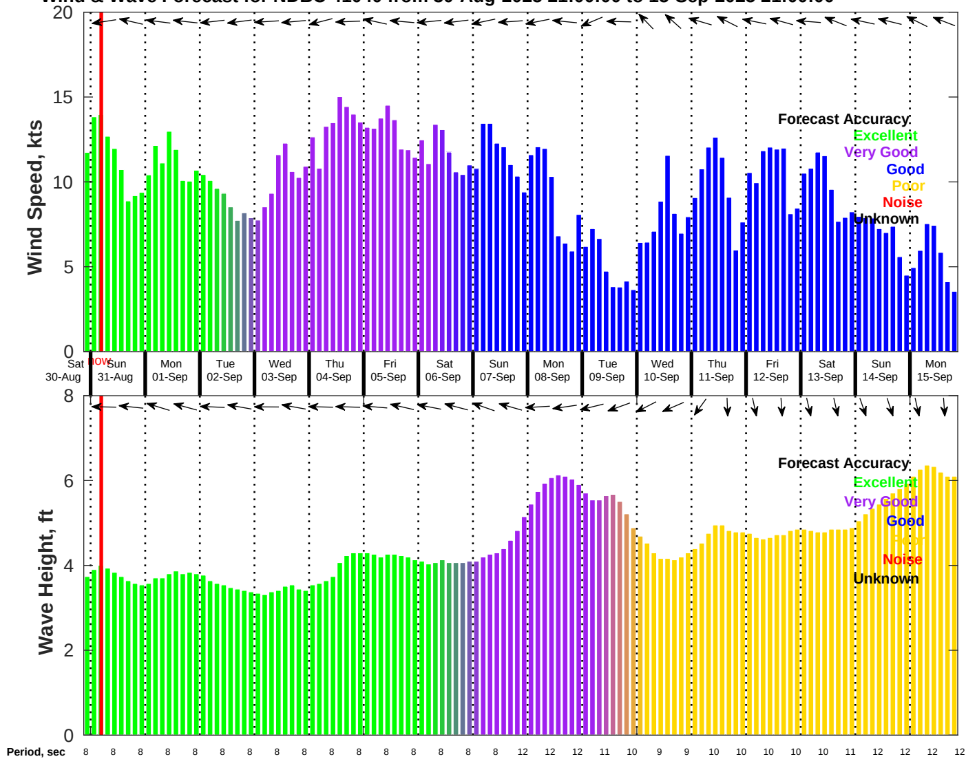
Wind & Wave Forecast for NDBC 41040 from 30-Aug-2025 21:00:00 to 15-Sep-2025 21:00:00
