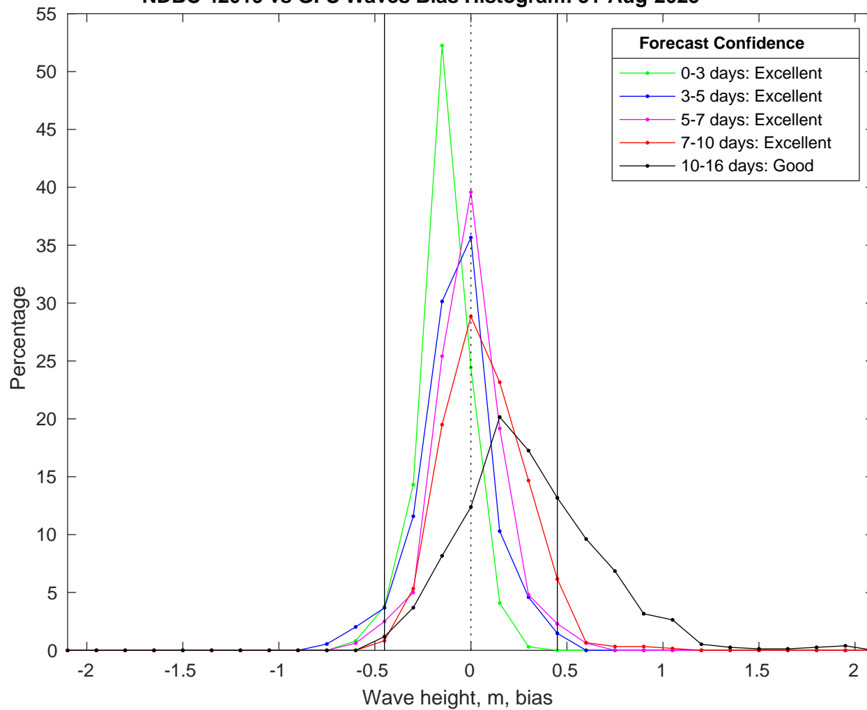
NDBC 42019 vs GFS Waves Bias Histogram: 31-Aug-2025
