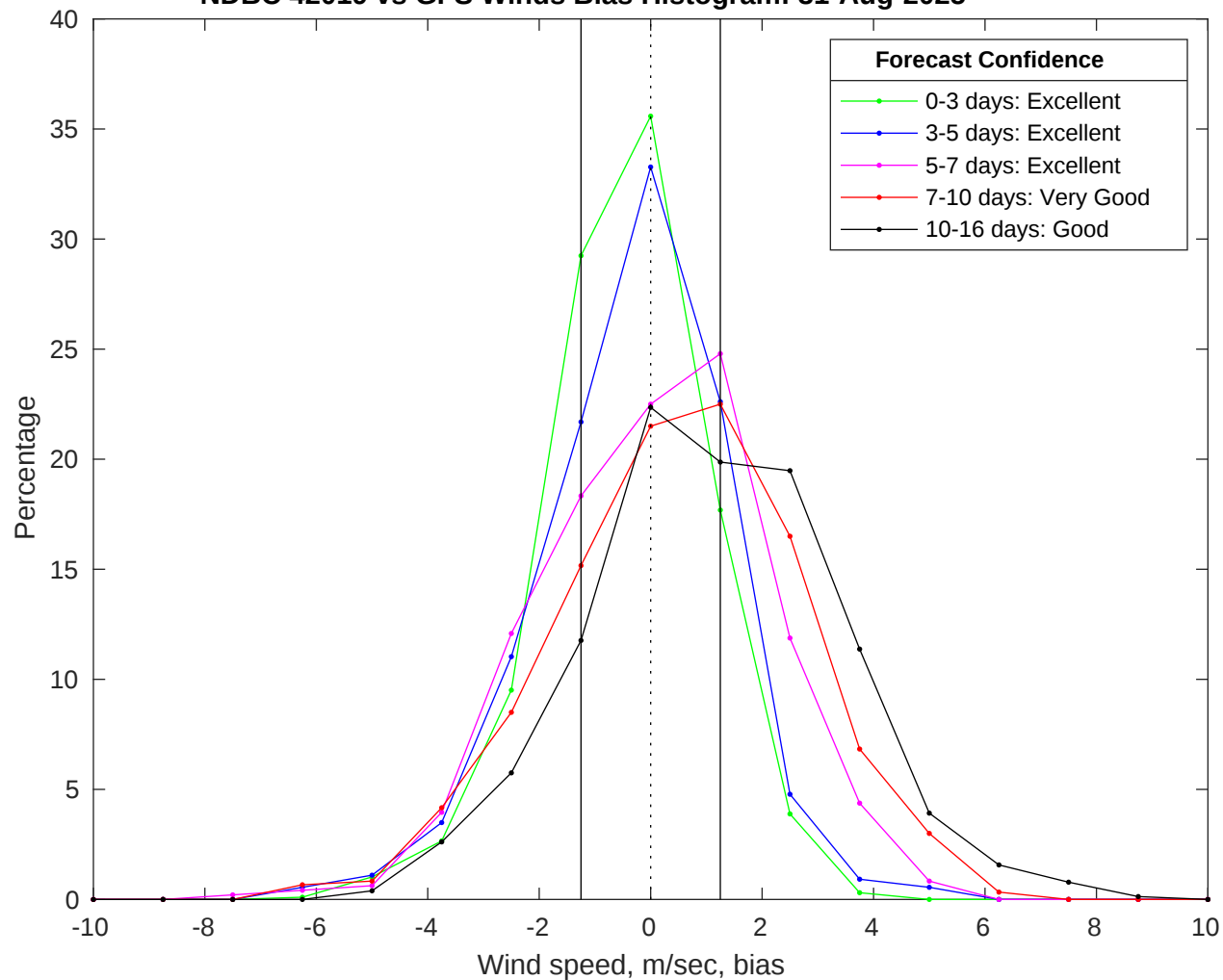
NDBC 42019 vs GFS Winds Bias Histogram: 31-Aug-2025
