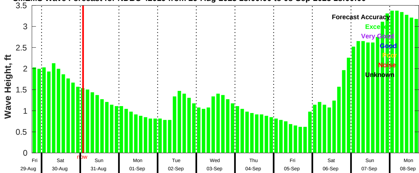
CMEMS Wave Forecast for NDBC 42019 from 29-Aug-2025 18:00:00 to 08-Sep-2025 18:00:00
