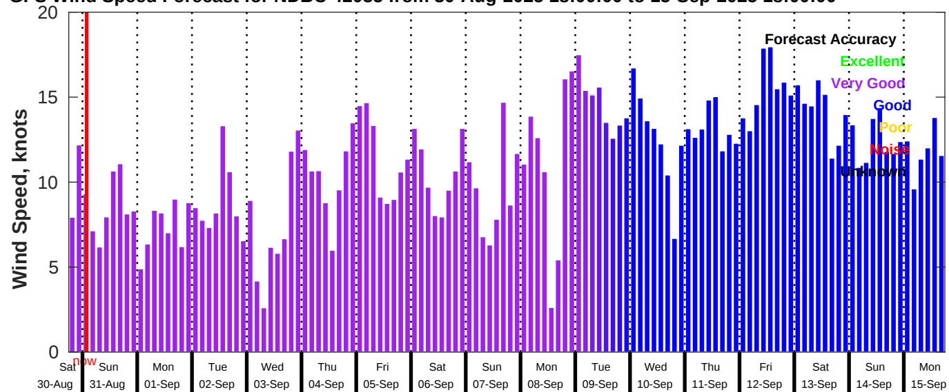
GFS Wind Speed Forecast for NDBC 42035 from 30-Aug-2025 18:00:00 to 15-Sep-2025 18:00:00
