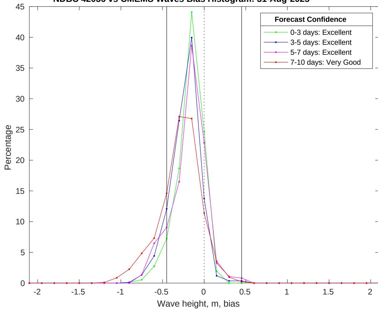
NDBC 42036 vs CMEMS Waves Bias Histogram: 31-Aug-2025
