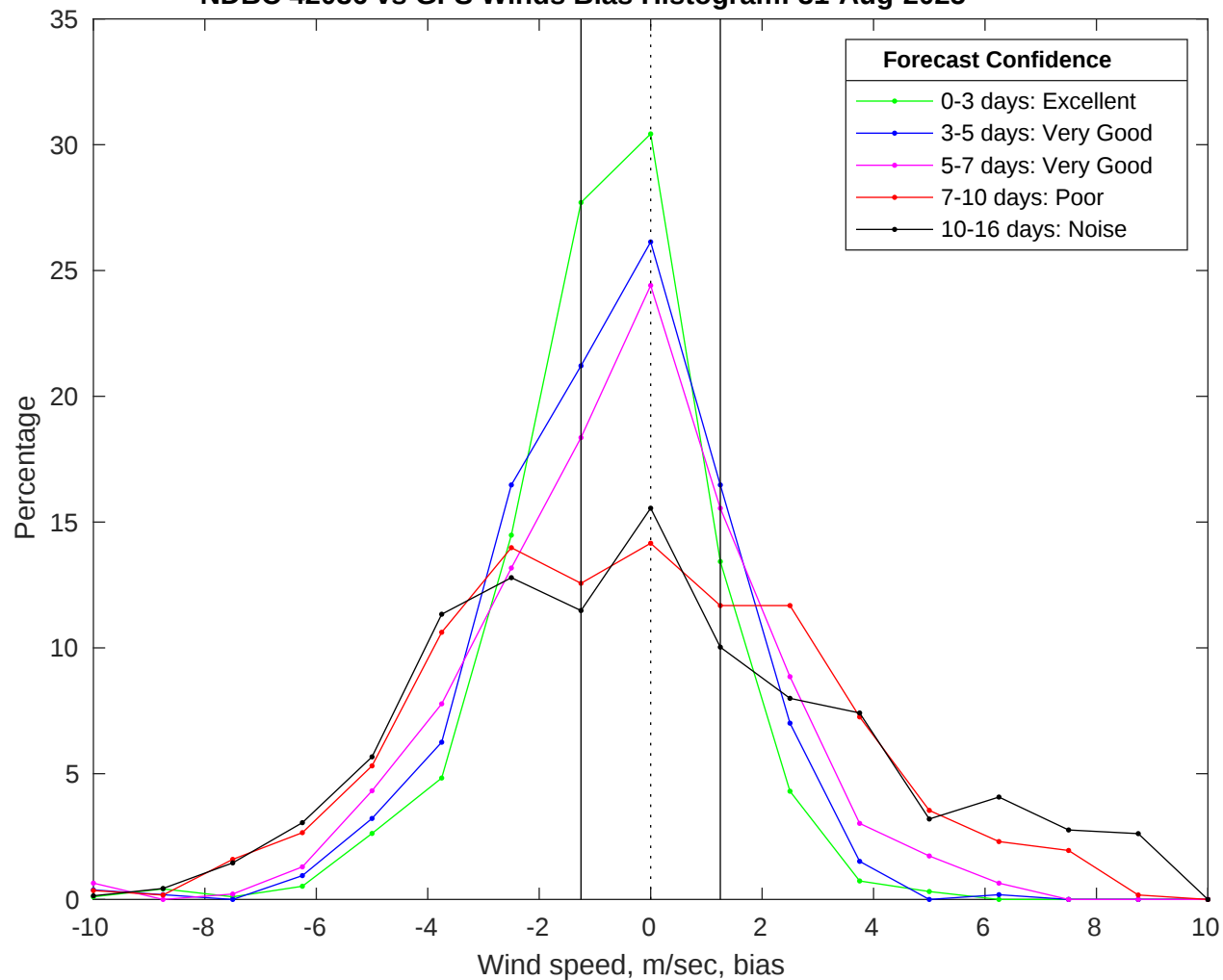
NDBC 42036 vs GFS Winds Bias Histogram: 31-Aug-2025
