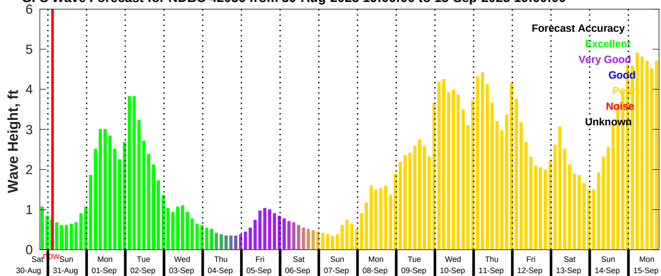
GFS Wave Forecast for NDBC 42036 from 30-Aug-2025 19:00:00 to 15-Sep-2025 19:00:00
