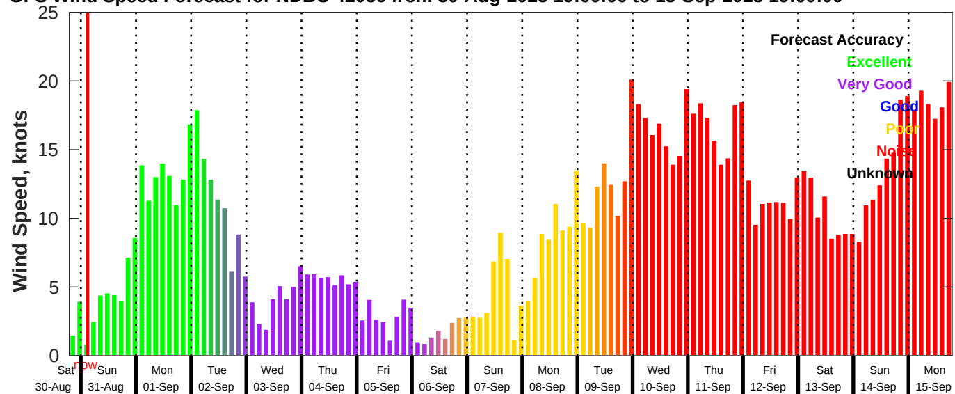
GFS Wind Speed Forecast for NDBC 42036 from 30-Aug-2025 19:00:00 to 15-Sep-2025 19:00:00
