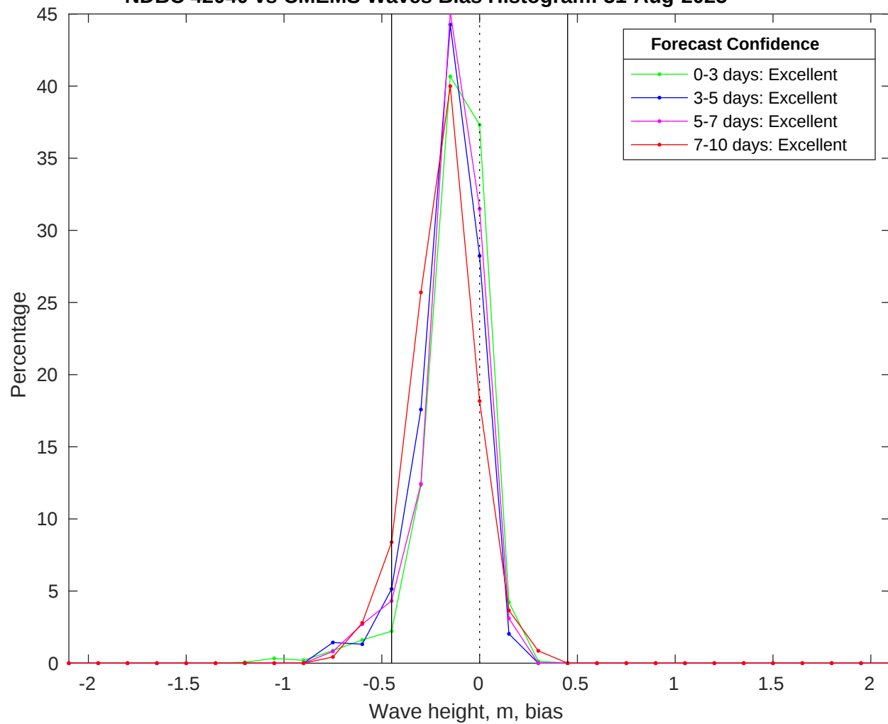
NDBC 42040 vs CMEMS Waves Bias Histogram: 31-Aug-2025
