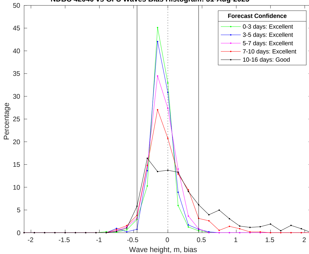
NDBC 42040 vs GFS Waves Bias Histogram: 31-Aug-2025
